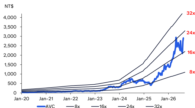
Figure 3. AVC - Forward P/E band
