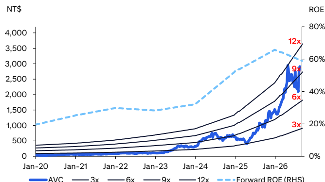
Figure 4. AVC - Forward P/B band
